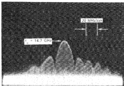
Fig. 4 Frequency Spectrum of Output Pulsed RF Signal from the Ku-Band Beacon Transponder (sin x/x)
