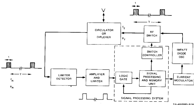
Fig. 1 Block Diagram of Cooperative Signal-Processing Beacon Transponder
