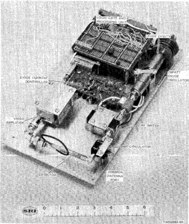
Fig. 2 14.5-GHz Solid-State Cooperative Beacon Transponder for Airport Surface Detection (ASD) Radar
