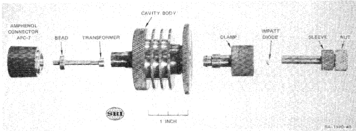
Fig. 3 Disassembled Ku-Band IMPATT Diode Oscillator
